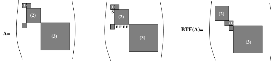
Figure 6: The initial matrix is not in BTF (left plot) and the ordering is not BTF compatible (factors in the middle plot). The ordering on the right is BTF compatible and preserves sparsity. F: fill-in. S: local symmetrization.
