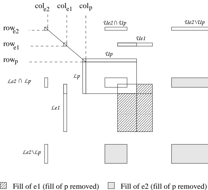
Figure 7: AMFI areas in the expanded matrix.
