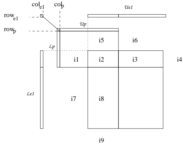
Figure 8: AMFI: different cases of local symmetrization. i1, i2, i3, i4, i5, i6 are cases encountered in loop 1 , i7, i8, i9 are cases encountered in loop 2 .
