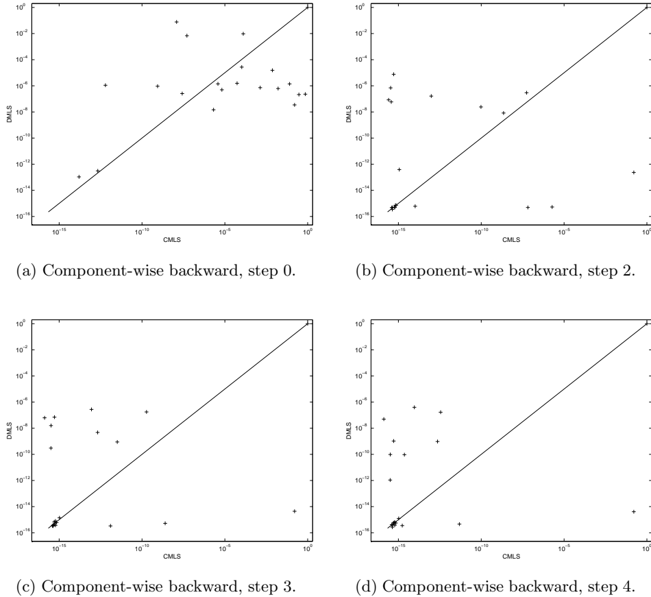
Figure 9: SuperLU_DIST component-wise backward error during iterative refinement.
