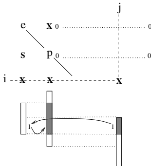
Figure 4: Effect of variable elimination in both directions on reducibility detection ( S indicates the position of local symmetrization).
