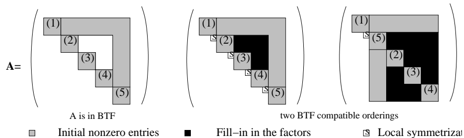
Figure 5: Illustration of two BTF compatible orderings of a matrix A in BTF. Using two-way variable elimination introduces fill-ins in the factors.
