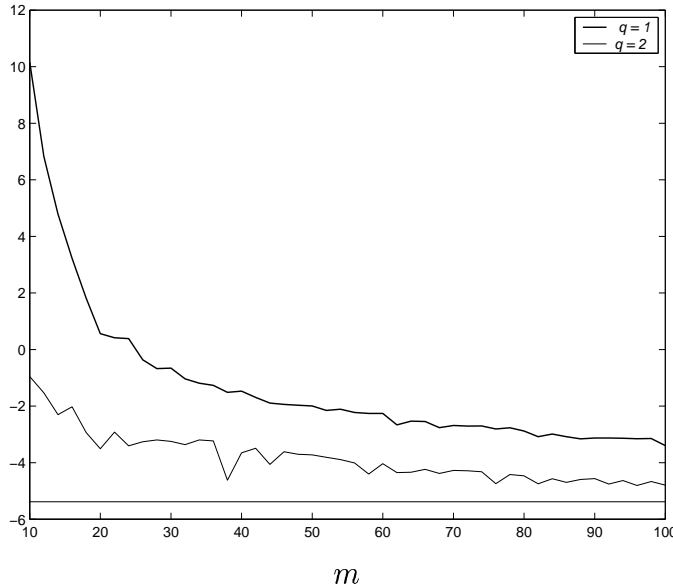
Figure 1: Departure from normality of matrix \mathcal{C}_A(m, q) as a function of m and q on a logarithmic scale; q denotes the number of columns of matrix L in (3) and m the degree of P_m(z) . The horizontal line points out the asymptotic value of D^2(\mathcal{C}_A(m, 2)) for large m .
