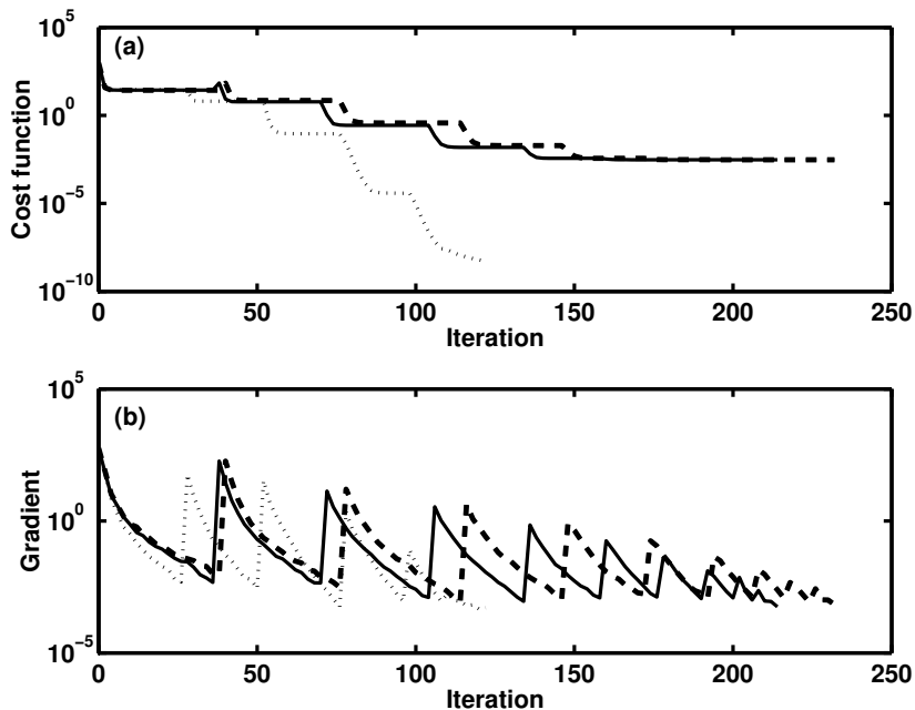
Figure 10. Case II: Convergence of (a) cost function and (b) gradient with inner loop at lower resolution. The solid line is for the tangent linear model and the dashed line for the perturbation forecast model. The dotted line shows for comparison the convergence using the tangent linear model at full resolution.
