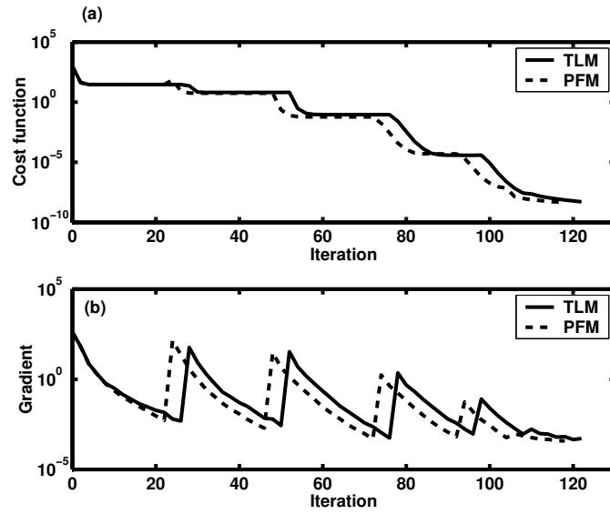
Figure 4. Case II: Convergence of (a) cost function and (b) gradient for tangent linear model (solid line) and perturbation forecast model (dashed line).
