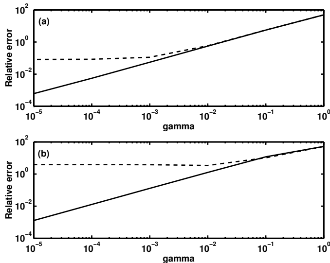
Figure 2. Plot of relative error E_R of u field against perturbation size for (a) Case I and (b) Case II. The solid line is for the tangent linear model and the dashed line for the perturbation forecast model.
