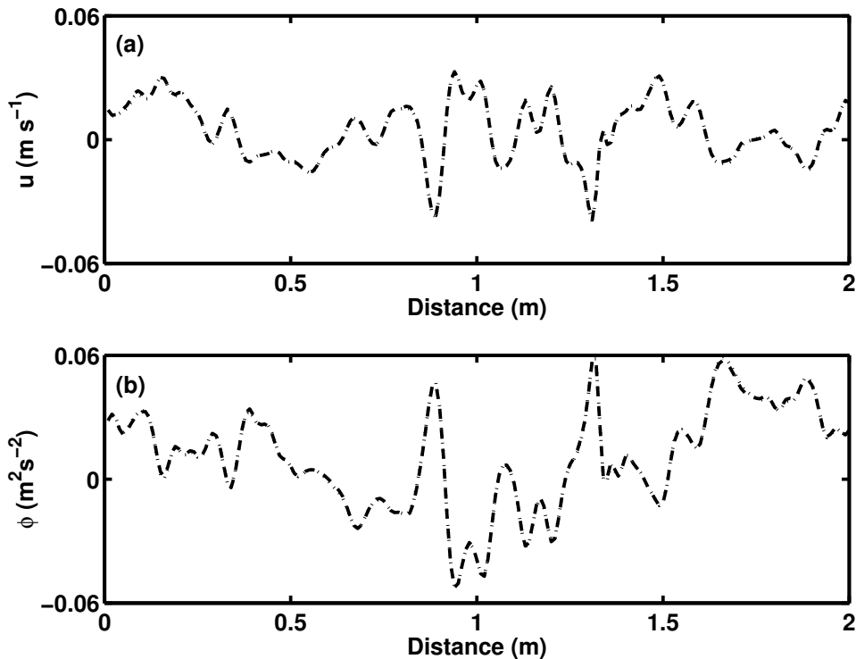
Figure 8. Case II: Analysis errors at the centre of the time window for (a) u field and (b) \phi field when noise is included on the observations. The dotted line indicates the assimilation using the TLM and the dashed line that using the PFM.
