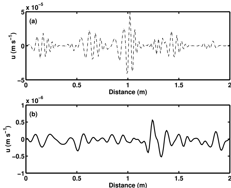
Figure 11. Case II: Analysis errors in u field at the centre of the time window using a low resolution inner loop. Plot (a) shows the analysis error, with the dotted line indicating the assimilation using the TLM and the dashed line using the PFM. Plot (b) shows the difference between the two analyses
