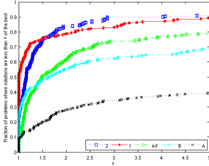
FIG. 4.1. Performance profiles for the condition number estimates for 245 matrices. A marks the condition number estimate of the original matrix; B marks that of Bunch’s algorithm [2]; inf , 1, and 2 mark that of the parallel scaling algorithm with \infty -, 1-, and 2-norms (with at most 25 iterations). At, for example \tau = 3 , the curves from top to bottom correspond to the labels given in the legend from left to right.
