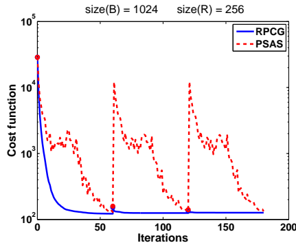
Figure 6: The cost function versus the inner iterations. The experiments consists in 3 Gauss-Newton iterations with 60 inner iterations.
