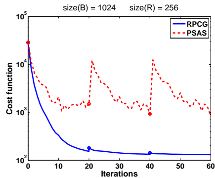
Figure 4: The cost function versus the inner iterations. The experiments consists in 3 Gauss-Newton iterations with 20 inner iterations.
