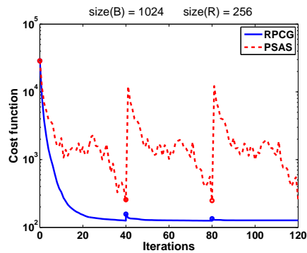
Figure 5: The cost function versus the inner iterations. The experiments consists in 3 Gauss-Newton iterations with 40 inner iterations.
