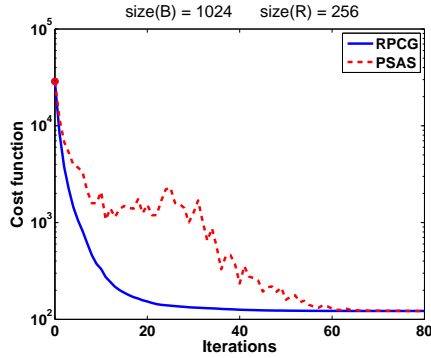
Figure 3: The cost function versus the inner iterations for 1 Gauss-Newton iteration.
