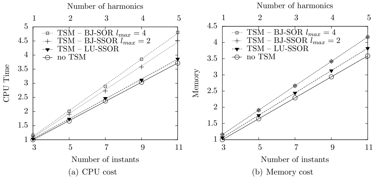
Figure 3. Costs of the different implicitation strategies.
