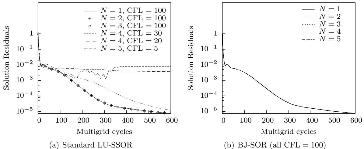
Figure 1. Convergence of computations.
