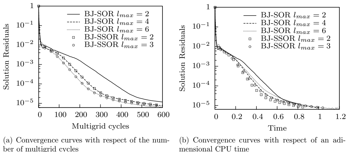
Figure 2. Effect of the number of modified LU-SSOR steps on convergence (all CFL = 100).
