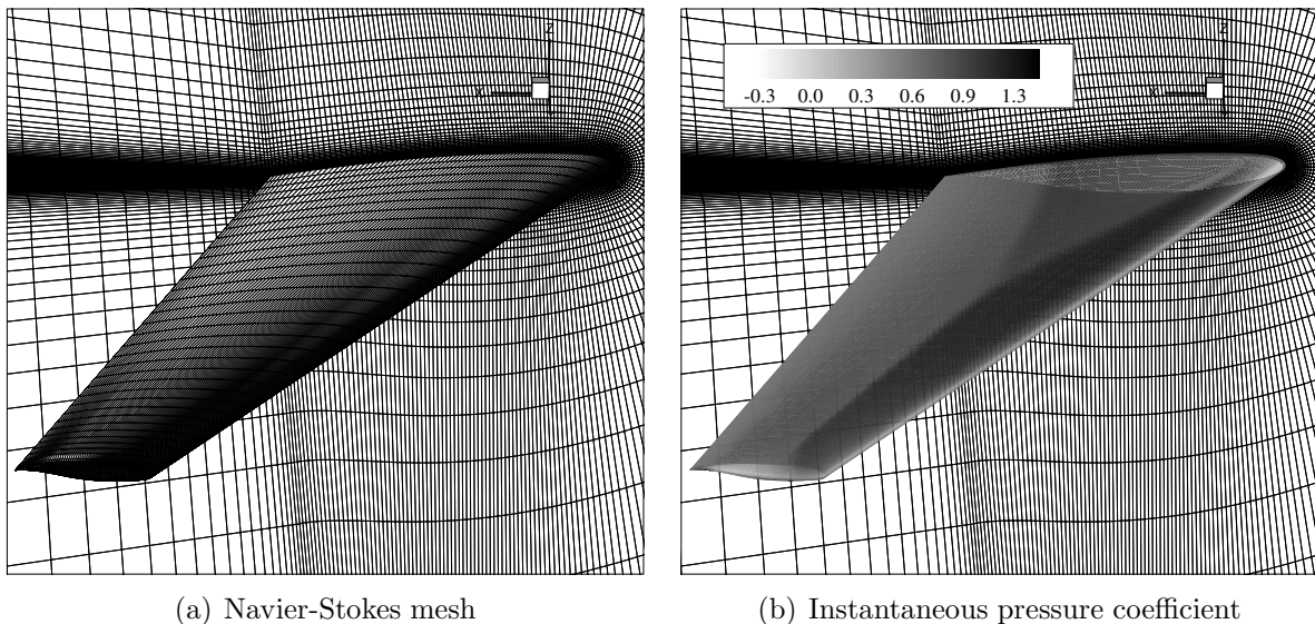
Figure 4. LANN Wing.
