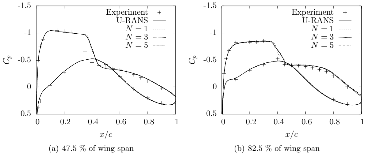
Figure 5. Time average of the wall pressure coefficient C_p .
