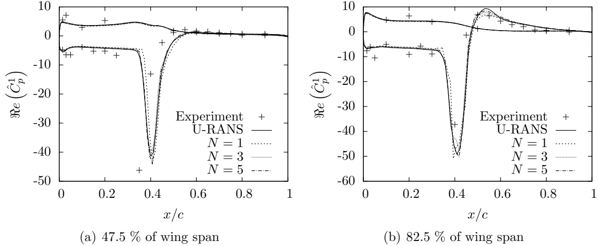
Figure 6. Real part of the first harmonic of C_p .
