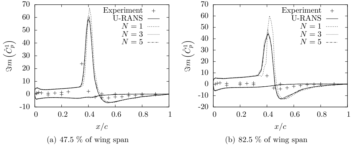
Figure 7. Imaginary part of the first harmonic of C_p .
