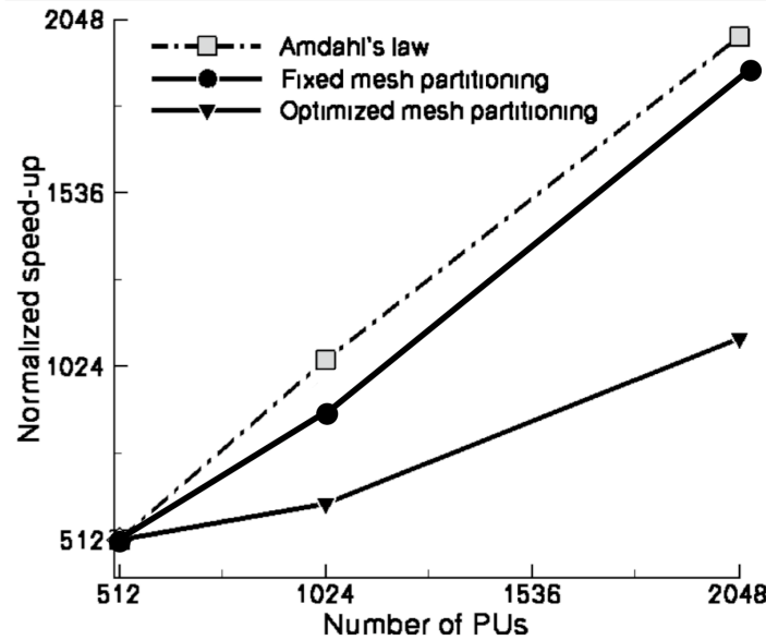
Fig. 2 Effect of the mesh partitioning strategy on the speed-up (optimized mesh-partitioning and fixed mesh partitioning with the elsA flow solver).
