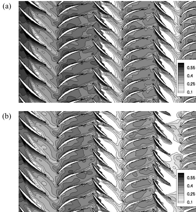
Fig. 13 Instantaneous flow fields of axial velocity computed with elsA at design (a) and off-design (b) operating conditions in a multistage compressor (near the casing, h/H=83\% ).
