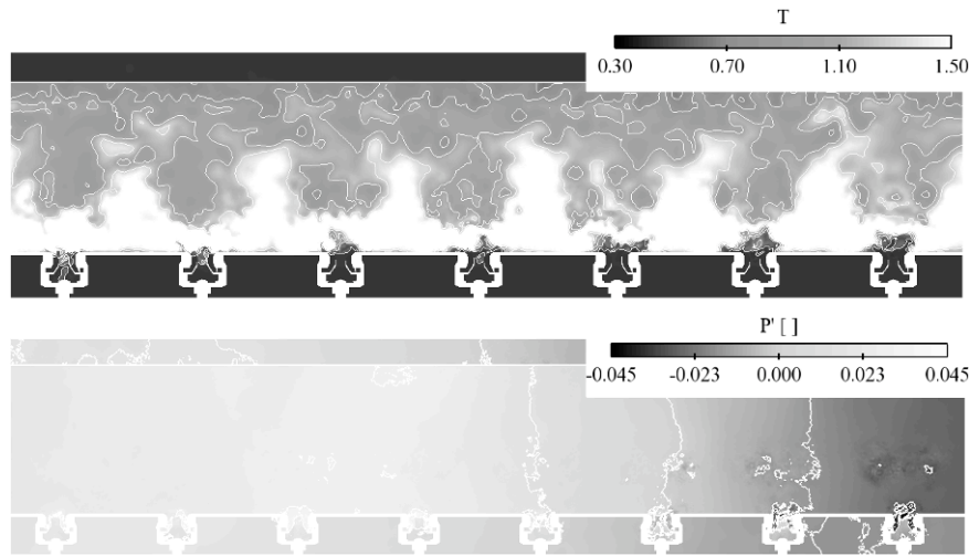
Fig. 8 Typical snapshot computed with AVBP (LES) for the configuration pictured on Fig. 7. The view is produced for a given radial plane going through all swirlers at a given instant (only few burners are pictured for clarity).
