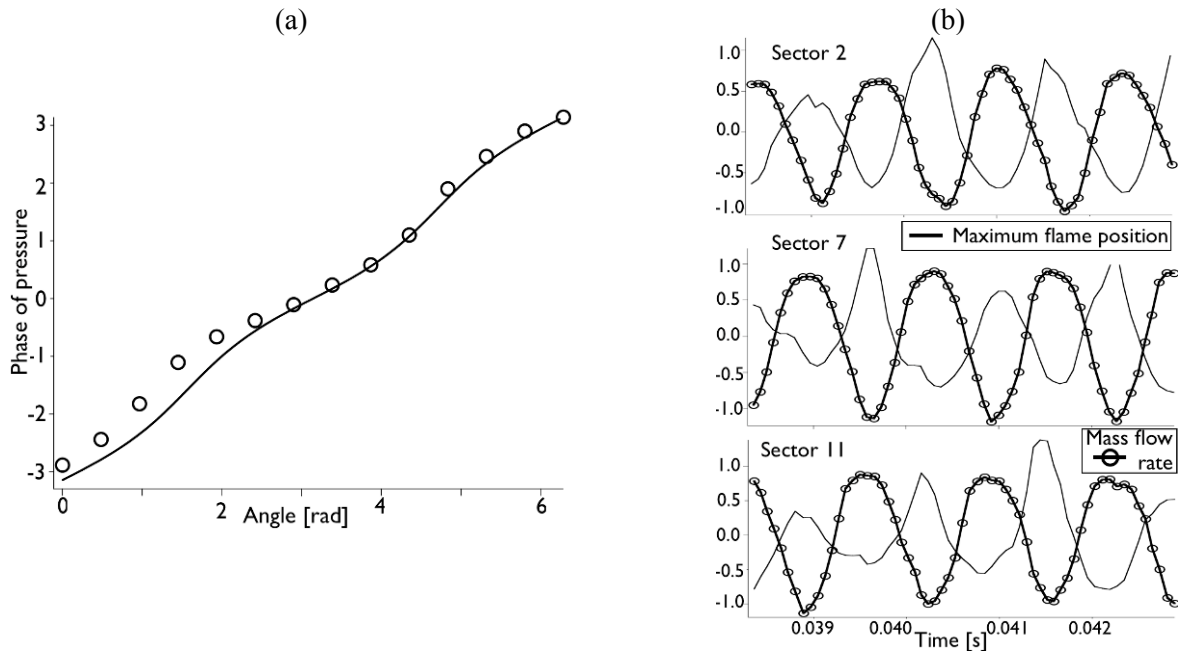
Fig. 9 Thermo-acoustic analysis of the LES results obtained with AVBP for the full annular aeronautical gas-turbine combustion chamber - (a) phase-angle relationship of the azimuthal pressure signal (symbols: analytical model, curve: LES data) and (b) swirled mass flow rate and axial flame position.
