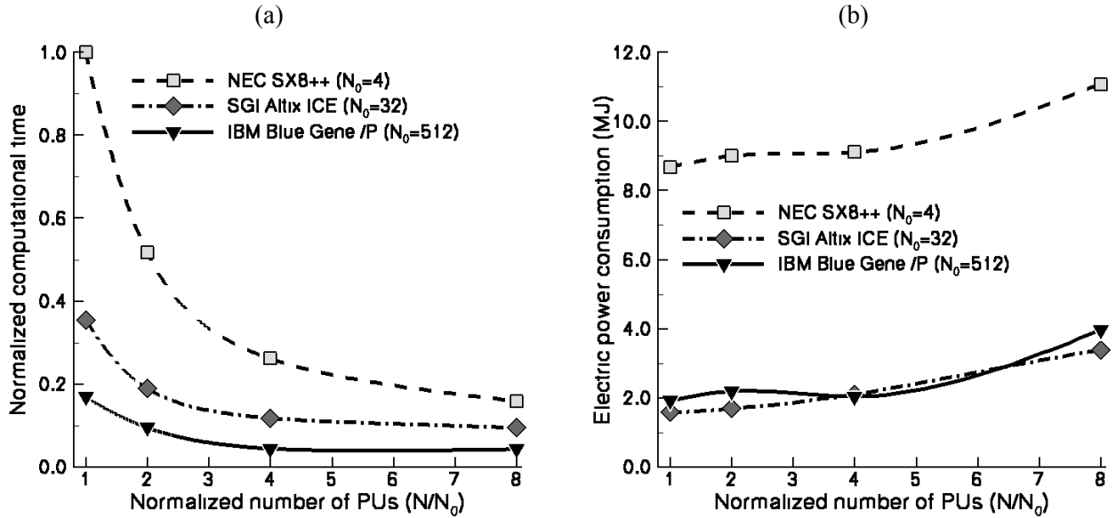
Fig. 3 Comparisons of the time needed to compute one iteration (a) and electric consumption (b) with the elsA flow solver: application to an industrial multistage compressor.
