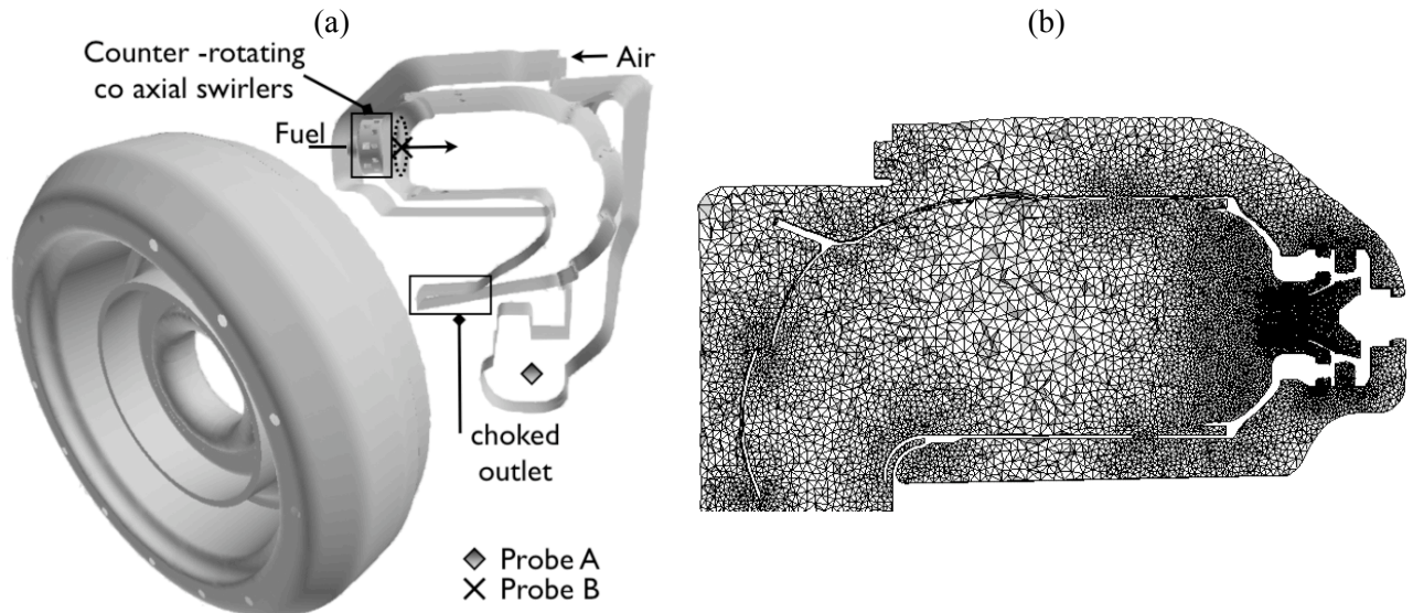
Fig. 7 Full annular aeronautical burner computed with AVBP (LES) for a thermo-acoustic analysis of the burner: (a) computational domain and (b) typical mesh resolution in the injector region.
