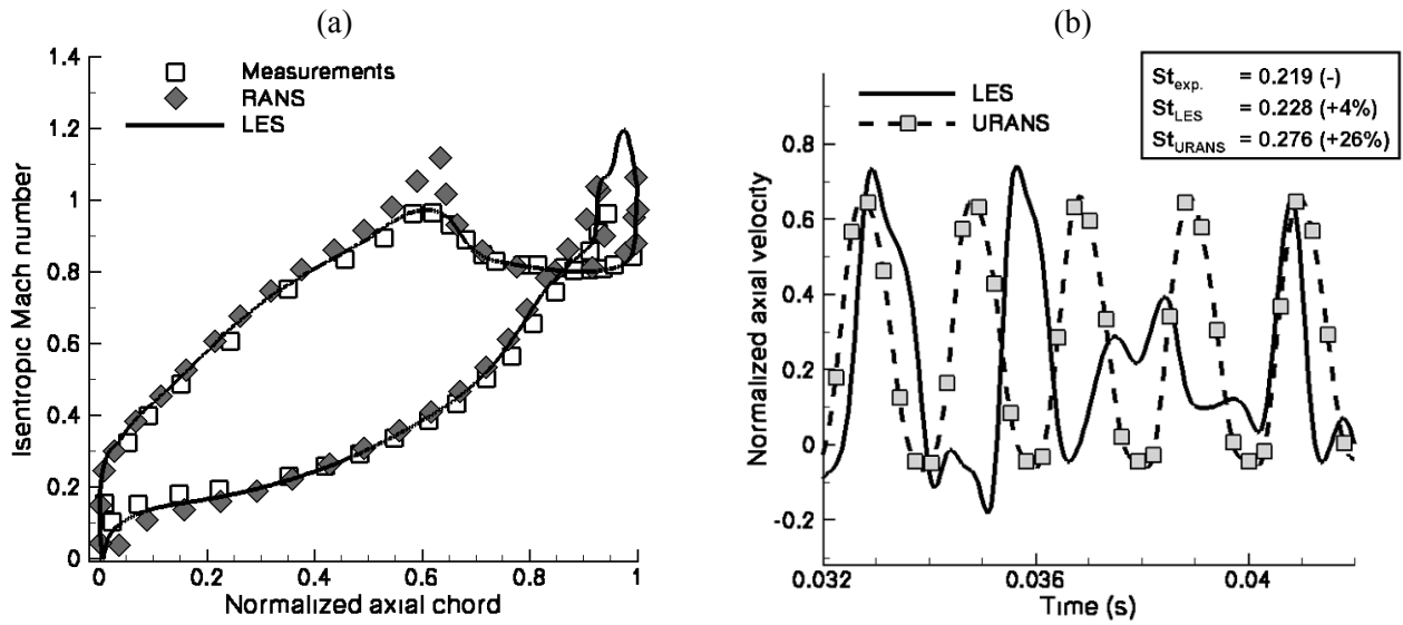
Fig. 15 Vortex shedding simulations performed with elsA behind the turbine IGV – comparisons of the isentropic Mach number (a) and unsteady axial velocity signals (b).
