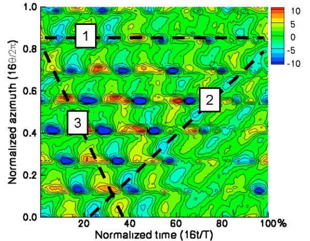
Fig. 12 Fluctuation of velocity angle \alpha' (in degrees ^{\circ} ) at section 280 and at design operating point (near the casing, h/H=83\% ): (a) URANS simulation( elsA ), (b) measurements.
