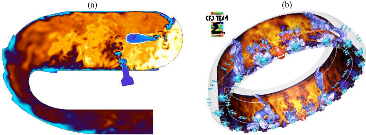
Fig. 6 Instantaneous temperature flow fields obtained with AVBP (LES) in aero-engine combustion chambers - (a) Turbomeca single sector chamber (Boudier et al. , 2007), (b) ignition sequence in a whole Turbomeca annular chamber (Boileau et al. , 2008).
