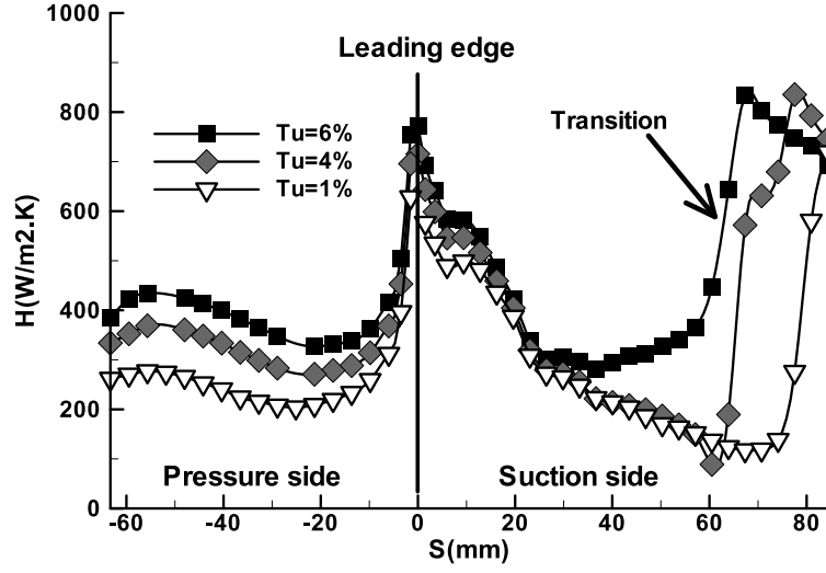
Fig. 16 Effect of the laminar to turbulent transition on the heat transfer coefficient H (IGV configuration, Arts, 1990).
