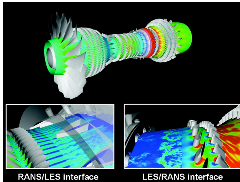
Fig. 1 Simulation of a whole gas turbine using RANS/LES coupling (van der Weide, 2008).
