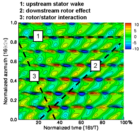
Fig. 12 Fluctuation of velocity angle \alpha' (in degrees ^{\circ} ) at section 280 and at design operating point (near the casing, h/H=83\% ): (a) URANS simulation( elsA ), (b) measurements.
