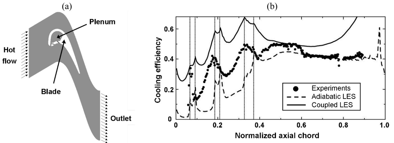
Fig. 17 Aero-thermal simulation of a cooling turbine blade (a) and time-averaged solution of cooling efficiency (b) obtained with LES (AVBP simulations).
