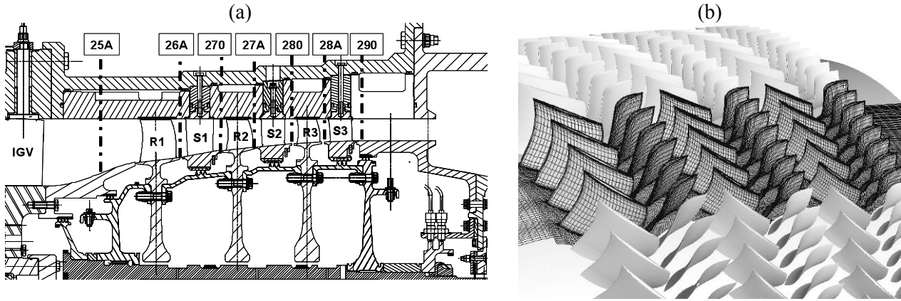
Fig. 10 View of the experimental compressor (a) and the numerical domain (b).
