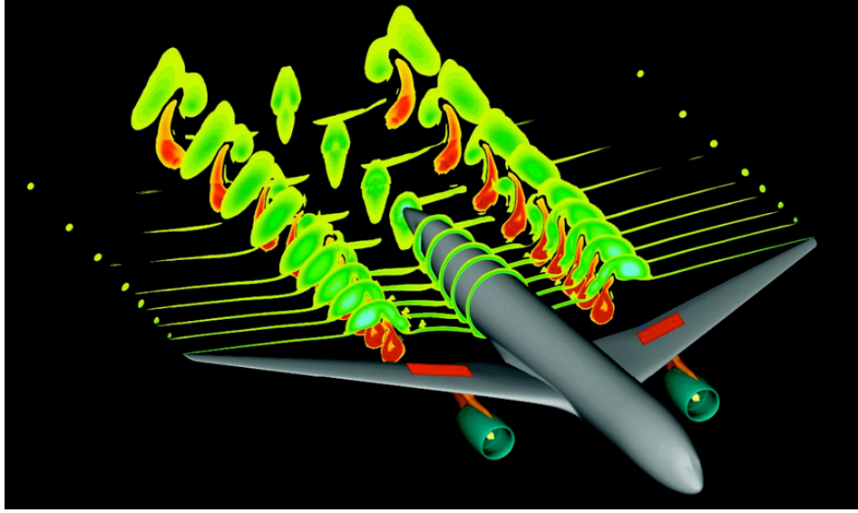
Fig. 5 Simulation of aero-elastic effects in a whole generic long-range aircraft performed with elsA – instantaneous solution of total pressure.
