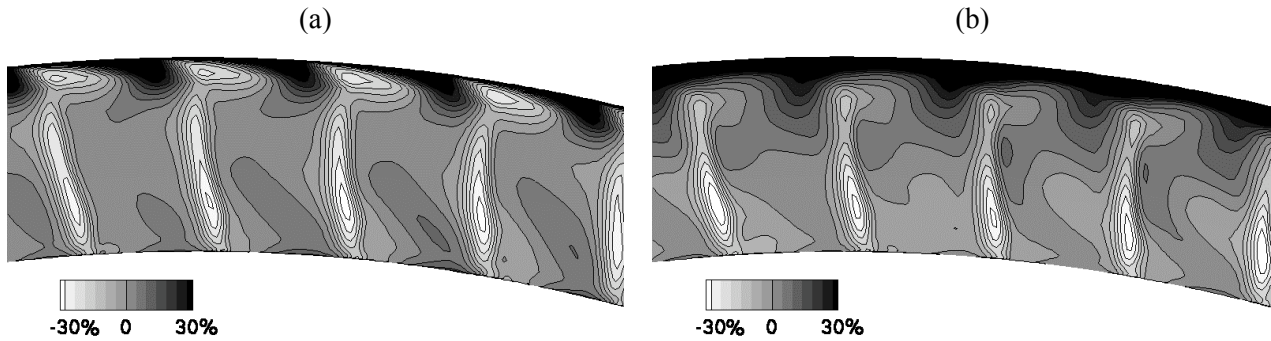
Fig. 11 Relative differences measured on mean values of axial velocity at design (a) and off-design (b) conditions between the unsteady and the steady RANS methods (third stage, elsA ).
