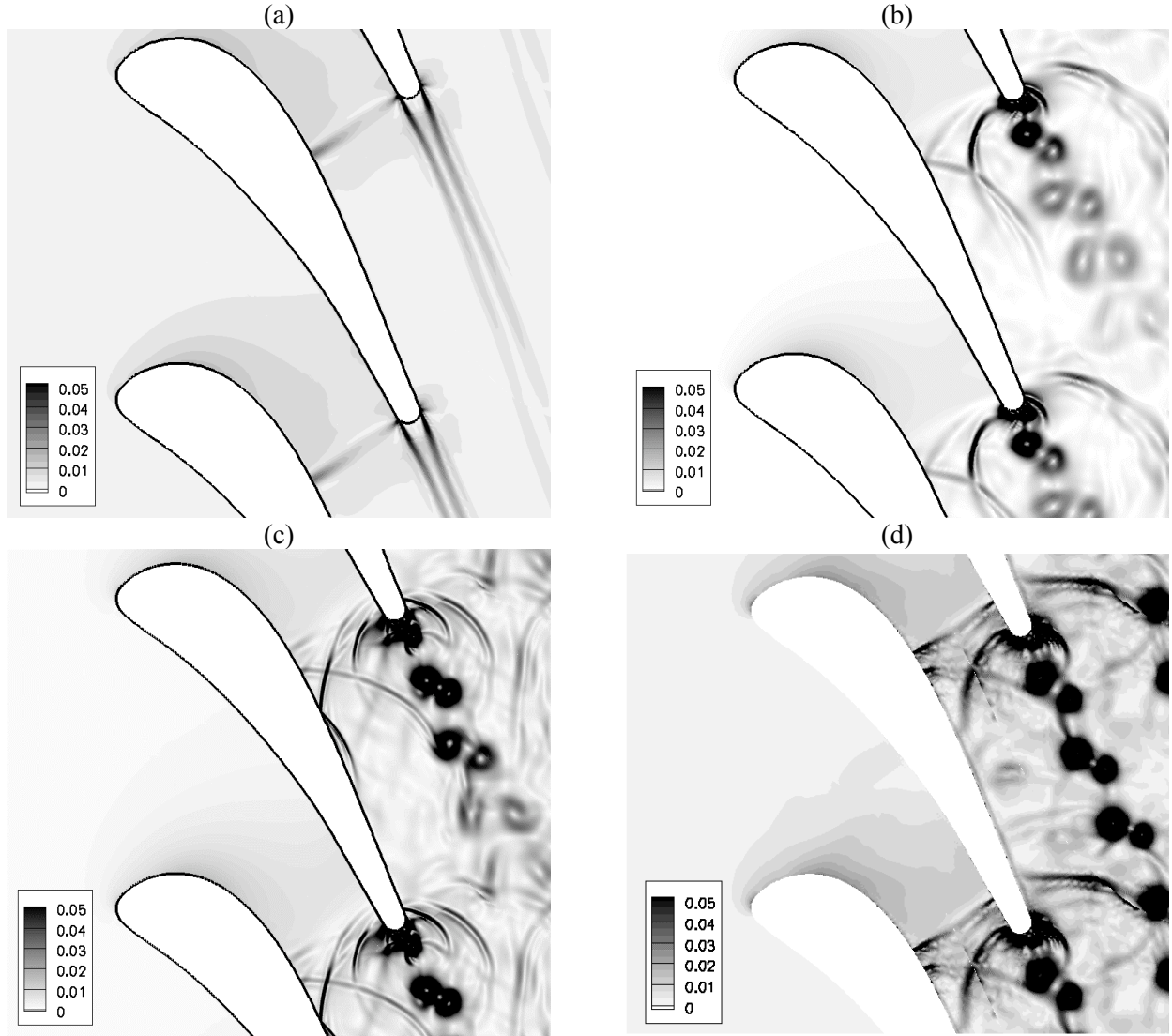
Fig. 14 Comparisons of instantaneous flow field of \text{grad } \rho in the IGV of a high-pressure turbine – RANS with elsA (a), URANS with elsA (b), LES with elsA (c), LES with AVBP (d).
