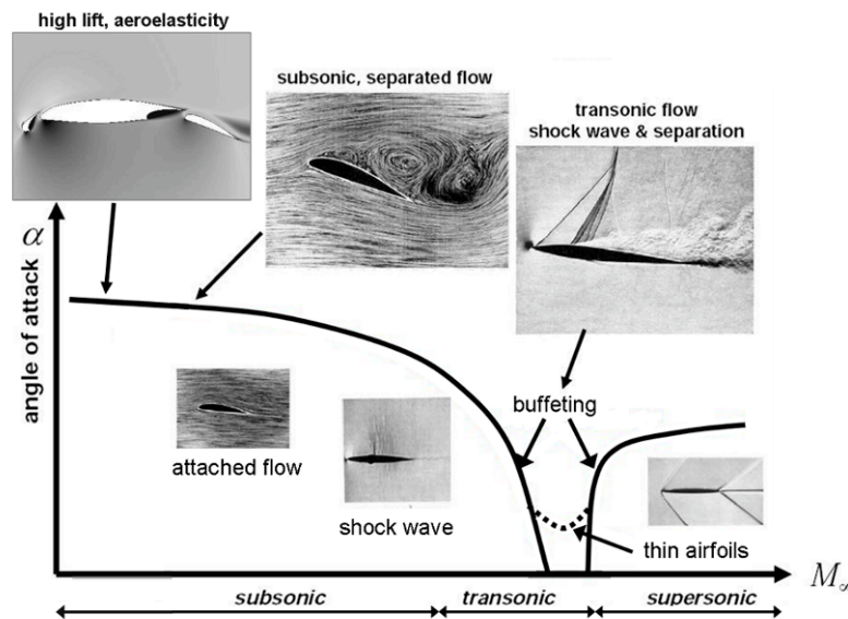
Fig. 4 Overview of the flow phenomena, depending on the flight conditions (Rossow and Kroll, 2008).
