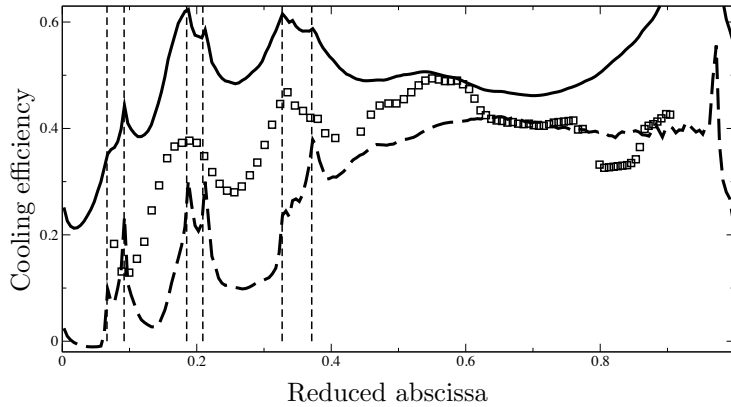
Figure 12. Cooling efficiency \Theta versus abscissa on the pressure side at steady state. Dashed line: adiabatic LES, solid line: coupled LES, symbols: experiment from UNIBW, vertical dashed lines: position of the holes.
