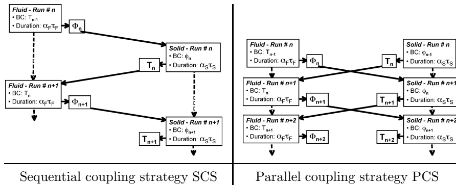
Figure 1. Main types of coupling strategies.
