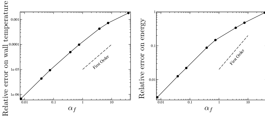
Figure 8. Flame/wall interaction simulation. Left: relative error on wall temperature ( x = 0 ) from t^+ = \delta_L^o t/s_L^o = 0 to t^+ = 82 , right: relative error on the energy fluxed into the wall on the same period.
