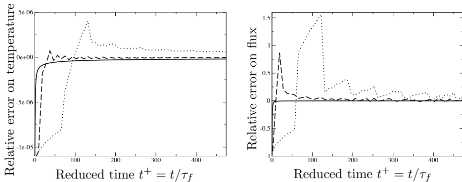
Figure 4. Tests of the PCS for the IFF case of Fig. 3. Effects of the coupling period between two events (measured by \alpha_s ). Left: relative error on wall temperature at x = 0 , right: relative error on wall flux at x = 0 . Solid line: \alpha_f = 0.131 , dashed: \alpha_f = 13.1 , dots: \alpha_f = 65.5 .
