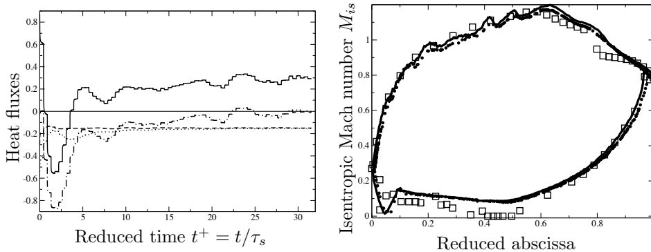
Figure 11. Time evolution of heat fluxes through the blade (left): external flux (solid line), plenum (dashed), holes sides (dot), sum of all fluxes (dot dashed). Isentropic Mach number along the blade (right): coupled LES (solid line), adiabatic LES (circles), experiment (squares).
