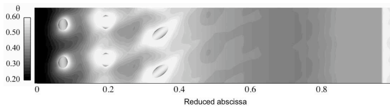
Figure 13. Spatial distribution of reduced temperature \theta on the pressure side of the blade. The computational domain is duplicated one time in the z direction.
